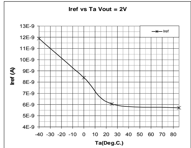
Typical Iref vs Ta Vout = 2V
